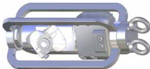
Type L 1200-2 with sledge for cleaning pipes with bends 35 mm S-arm, 2 nozzles max. 1200 bar / 150 l/min. Min. Pipe -Ø: 210 mm
